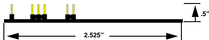
Figure 4 E*1941 One-Way Binary RF Module Dimensions
