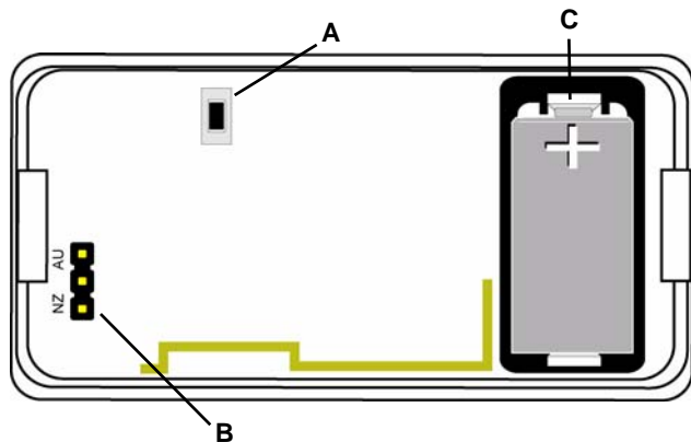
Figure 1 EN1224/EN1224-ON components
