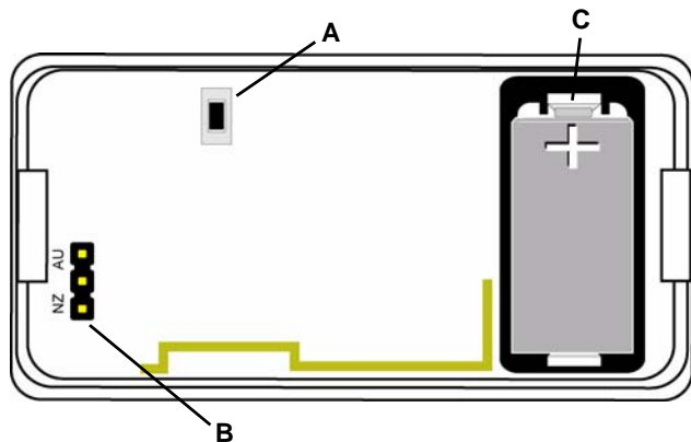
Figure 1 EN1236D components
