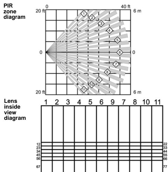
Figure 6 Mask zones
