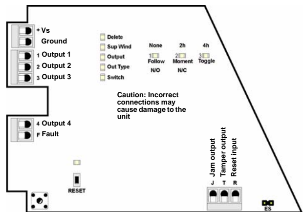
Figure 8 EE4204 Terminals
