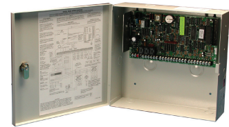
Security Panel DMP XR500 or DMP XR200 with DMP472 interface card
