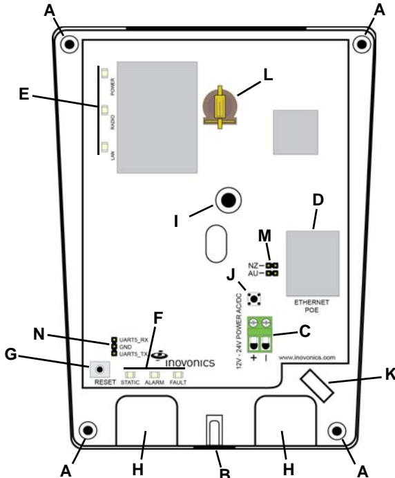
Figure 3 EN6080 area control gateway internal components
