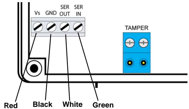
Figure 4 ACC653 serial data and power connections
