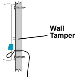
Figure 4 Mount the Transmitter to the Wall
