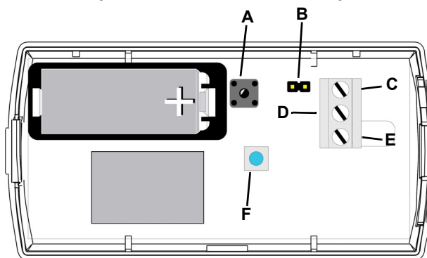
Figure 1 Dual input universal components
