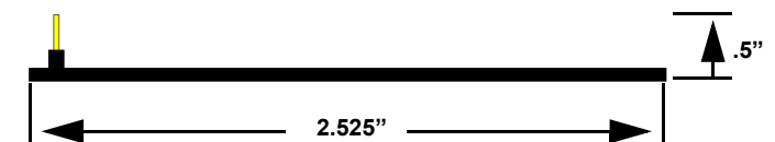
Figure 3 One-way serial RF module dimensions
