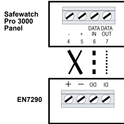
Figure 6 EN7290 receiver/interface to Safewatch Pro 3000 panel cabling
