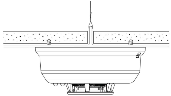
Figure 2 Mount the smoke detector across drop ceiling panel support
