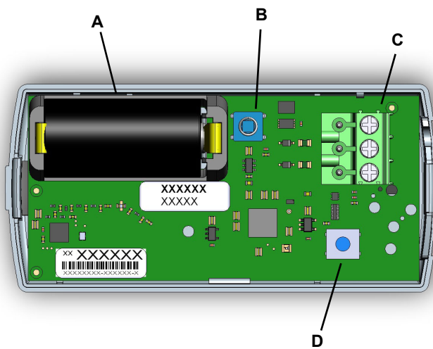
Figure 1 EN1501/EN1501-XL Components
