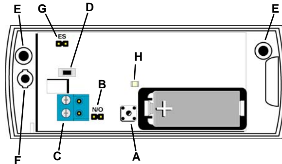
Figure 1 EE1215 components
