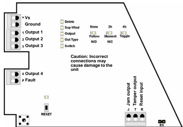
Figure 8 EE4204 Terminals
