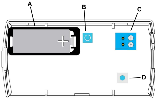
Figure 1 EN1501 Components
